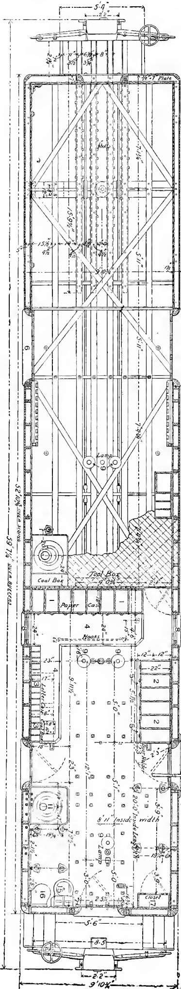
Fig. 600. Sectional Plan, Showing Underframing and Floor of 20-T. Mail Compartment. COMBINATION BAGGAGE AND MAIL CAR. NORFOLK & WESTERN RAILROAD.
